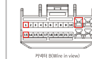
커넥터 B(Wire in view)
